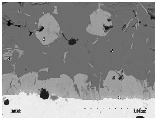
Fig. 6. The scanning picture of the AlSi5 silumin coat on pearlitic ductile iron with the marked points 1÷5 measuring the element concentration
