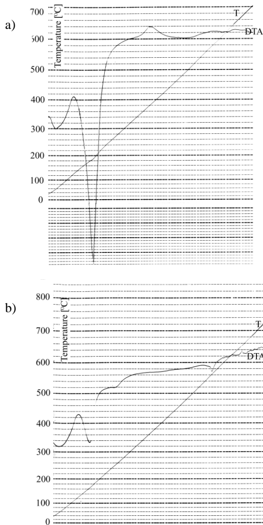
Fig. 4. Diagrams from derivatograph: a) waste gypsum (synthetic); b) gypsum GoldStar XL
