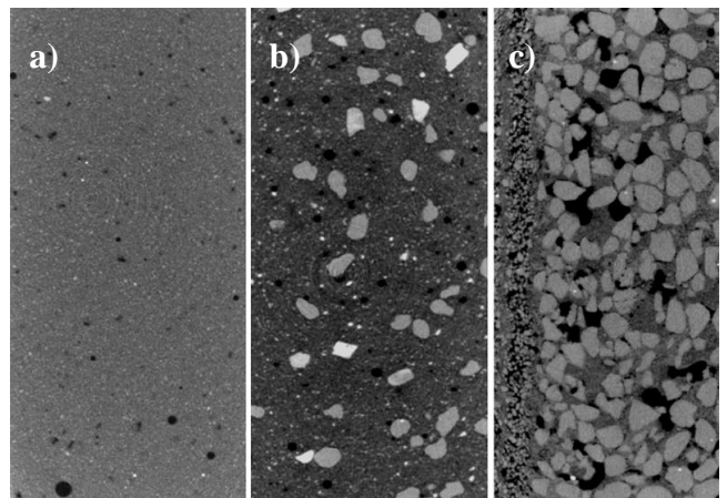
Fig. 6. Images from CT (Computed tomography) scan Metrotom 800: a) GoldStarXL gypsum mould b) synthetic gypsum mould, c) ceramic mould
