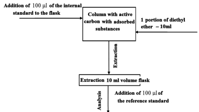
Scheme 1. Extraction process of compounds from the BTEX group from the column with active carbon
