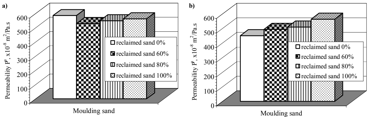
Fig. 3. Influence of the reclaim addition on the permeability, P^u , of the moulding sand of the following composition: high-silica sand 0 – 100 parts by mass, reclaim 0 – 100 parts by mass, GEOPOL binder 2.0 parts by mass, hardener – 14% of the binder amount: a) SA72, b) KR72
