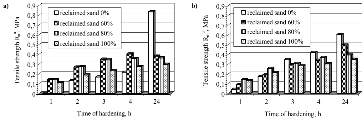
Fig. 1. Influence of the hardening time on the tensile strength, R_m^u of the moulding sand of the composition: high-silica sand 0 – 100 parts by mass, reclaim 0 – 100 parts by mass, GEOPOL binder 2.0 parts by mass, hardener – 14% of the binder amount: a) SA72, b) KR72
