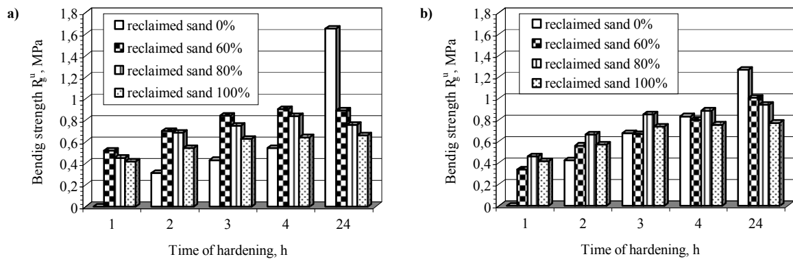
Fig. 2. Influence of the hardening time on the bending strength, R_g^u , of the moulding sand of the composition: high-silica sand 0 – 100 parts by mass, reclaim 0 – 100 parts by mass, GEOPOL binder 2.0 parts by mass, hardener – 14% of the binder amount: a) SA72, b) KR72
