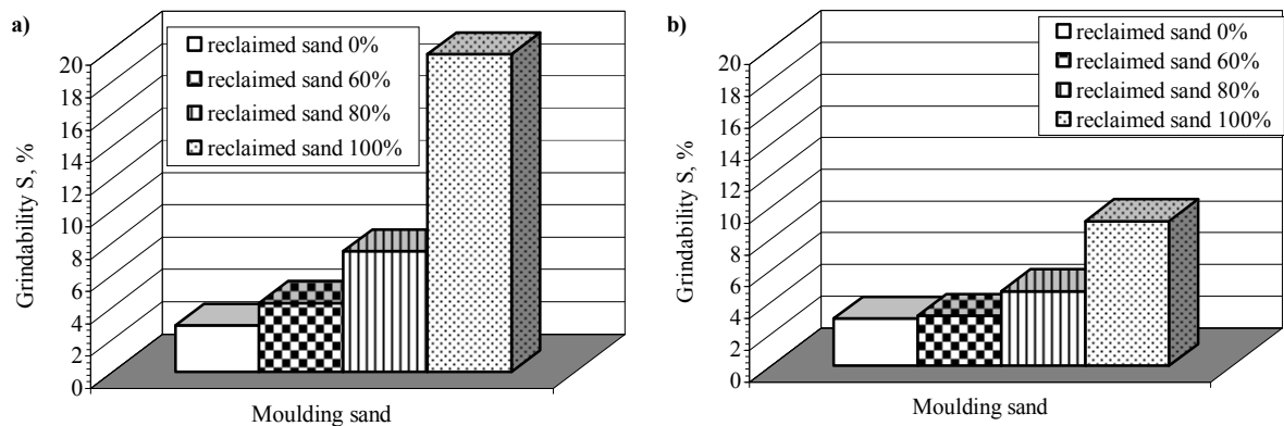
Fig. 4. Influence of the reclaim addition on the grindability, S of the moulding sands of the following composition: high-silica sand 0 – 100 parts by mass, reclaim 0 – 100 parts by mass, GEOPOL binder 2.0 parts by mass, hardener – 14% of the binder amount: a) SA72, b) KR72
