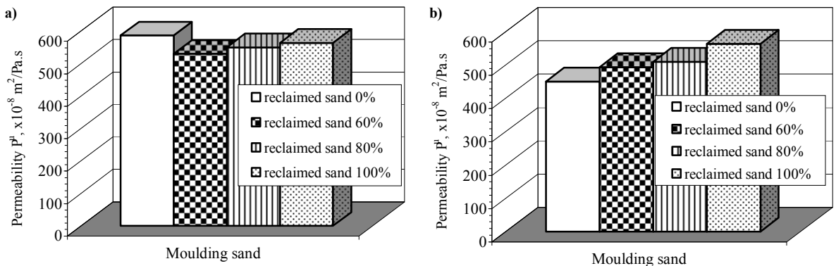
Fig. 3. Influence of the reclaim addition on the permeability, P^l , of the moulding sand of the following composition: high-silica sand 0 – 100 parts by mass, reclaim 0 – 100 parts by mass, GEOPOL binder 2.0 parts by mass, hardener – 14% of the binder amount: a) SA72, b) KR72
