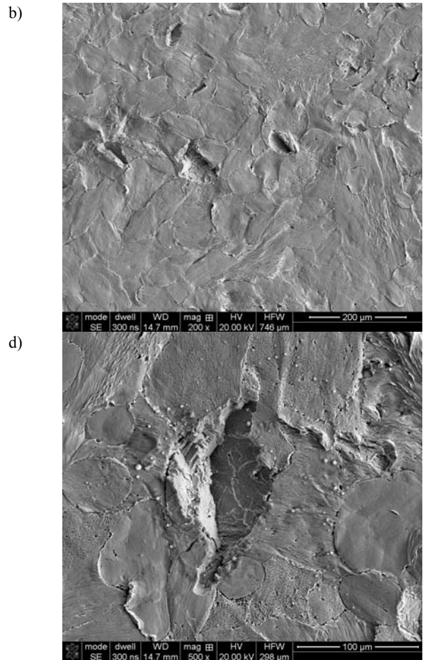
Fig. 5. SEM microphotographs showing surface changes in the ZnAl4 alloy upon the cavitation test carried out on the vibration stand a) depletion of \eta+\alpha eutectic in grain and phase boundaries zones, b), c) erosion of \eta solid solution dendrites and \eta + \alpha , d) fatigue striations
