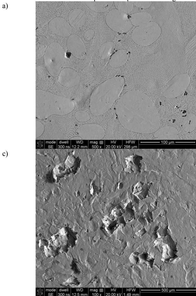
Fig. 5. SEM microphotographs showing surface changes in the ZnAl4 alloy upon the cavitation test carried out on the vibration stand a) depletion of \eta+\alpha eutectic in grain and phase boundaries zones, b), c) erosion of \eta solid solution dendrites and \eta + \alpha , d) fatigue striations
