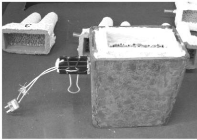
Fig. 1. Mould prepared for an experiment
