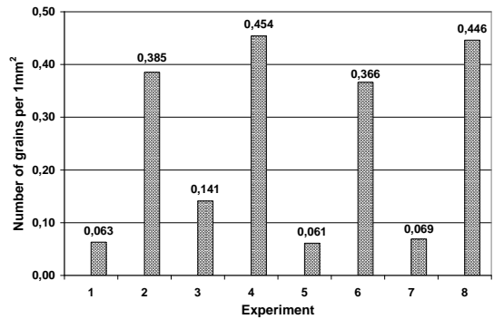
Fig. 4. Number of grains per 1\text{mm}^2 vs surface area
