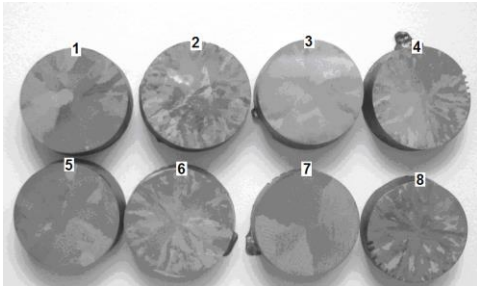
Fig. 3. Macrostructure on cross-sections of castings
