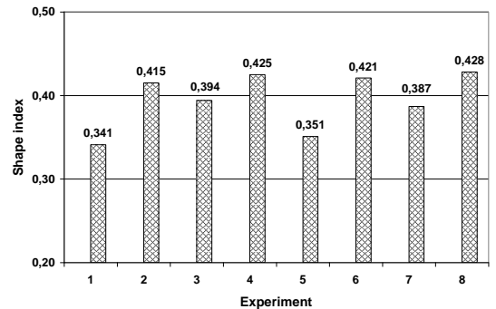
Fig. 6. A comparison of the mean grain shape index
