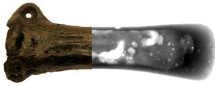
Fig. 8. X-ray image of axe No. NG24 together with the view of part of the artefact with visible defects
