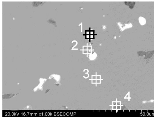
Fig. 12. The SEM images of the axle (NG21) microstructure with the EDS micro-areas spots (refer to table 2)
