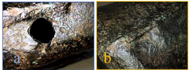
Fig. 7. Axe (No. NG26) with casting defects: incomplete filling - misrun (a) and flashes along the line joining the mould – casting seam (b)
