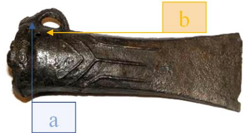
Fig. 5. Axe, visible remains of gating systems – marked in yellow (axe No. NG25)
